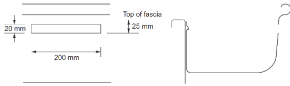
Figure 7.4.7c: Construction of front face weir
